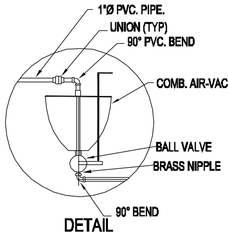
AIR RELEASE VALVE AND ROADWAY DETAIL
